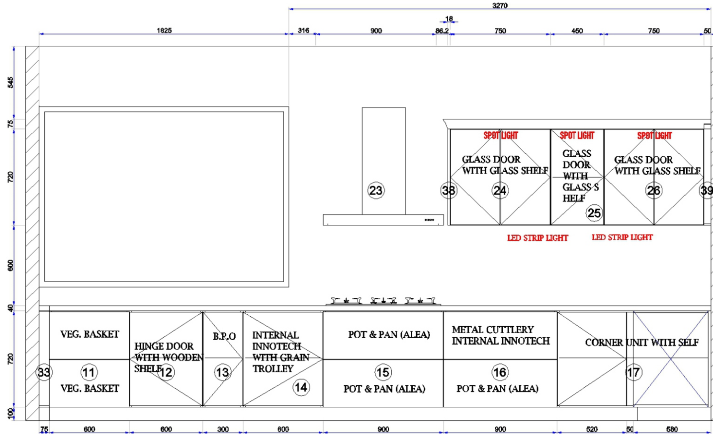
A View elevation drawing
