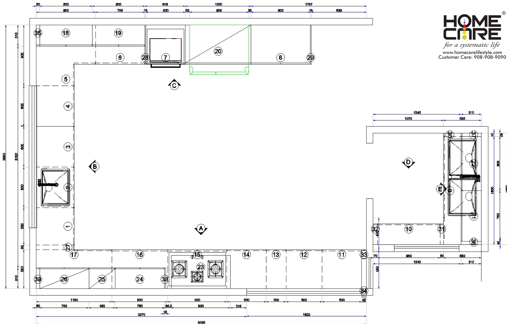
Plan drawing
