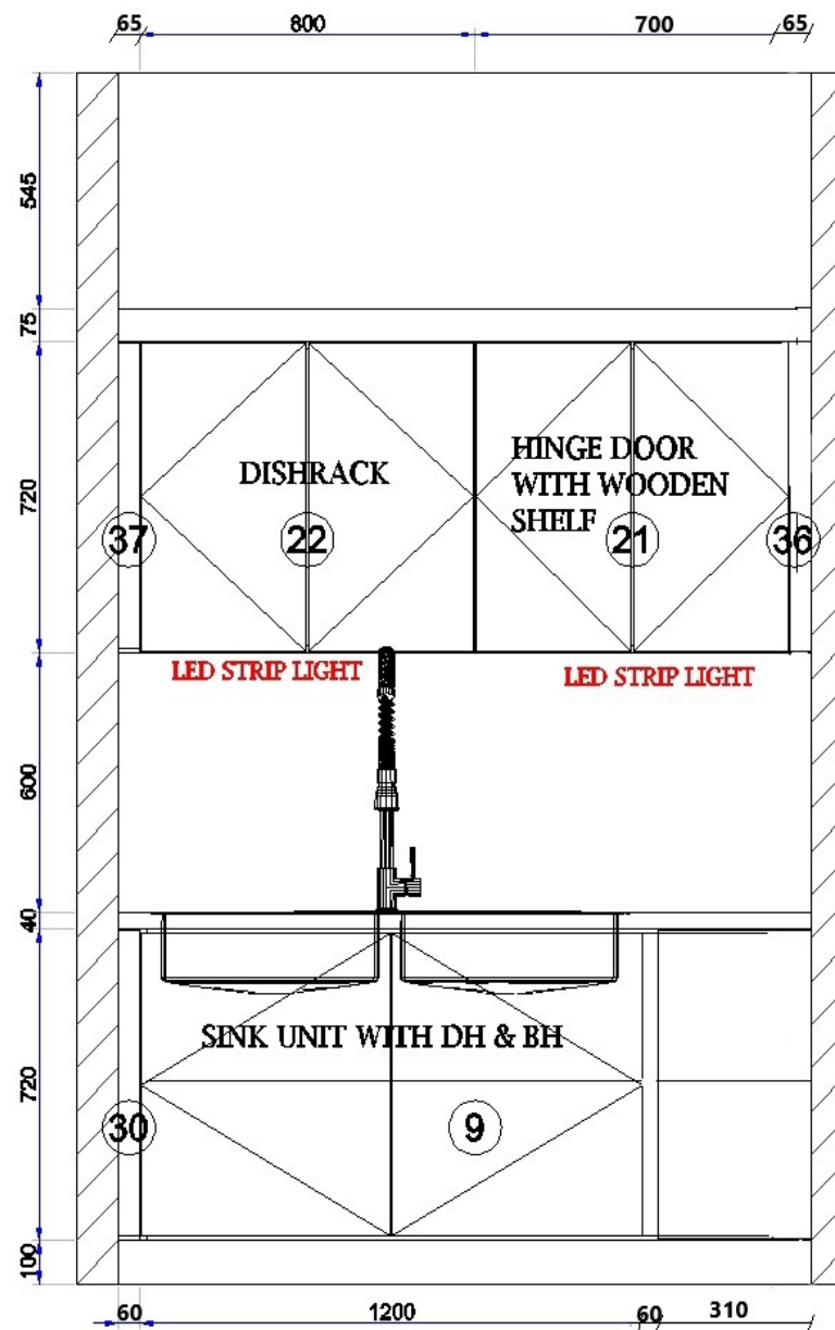
E View elevation drawing
