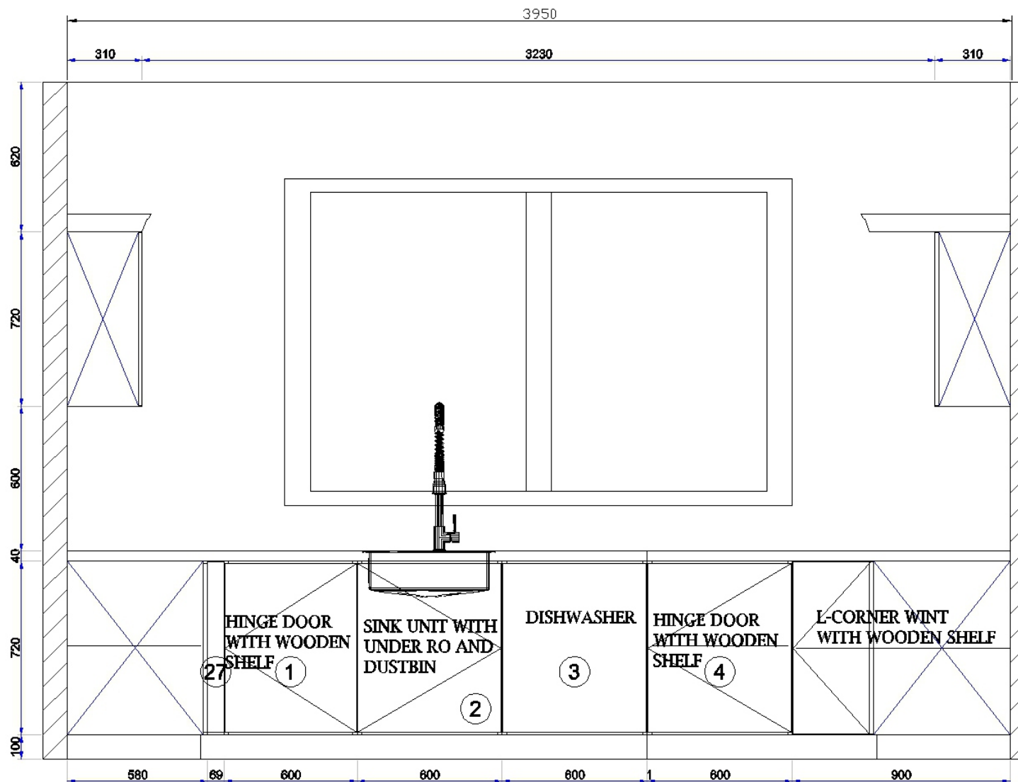
B View elevation drawing
