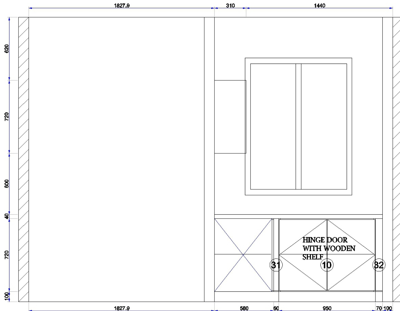
D View elevation drawing
