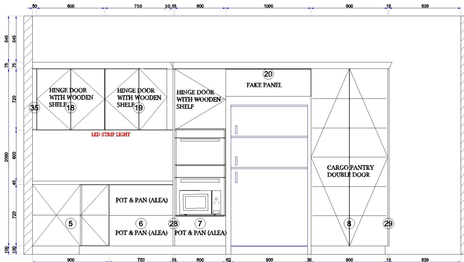
C View elevation drawing
